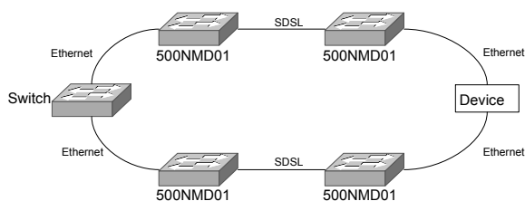
Abbildung 2: Typical topology for use with 500NMD01
